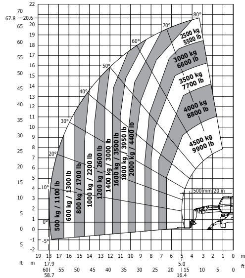
Rotation on stabilizers with 5000 kg winch
