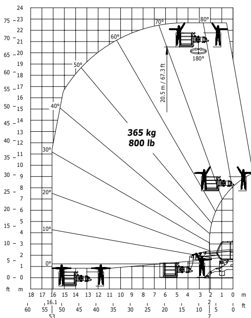
Rotation on stabilizers with 365 kg platform
