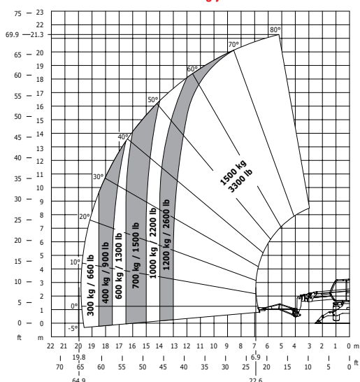
Rotation on stabilizers with 1500 kg jib
