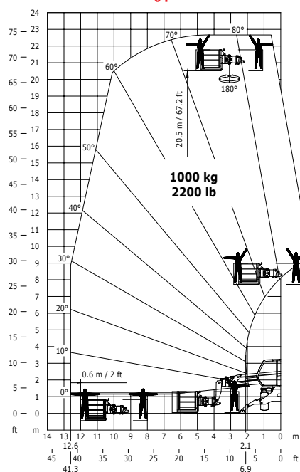
Rotation on stabilizers with 1000 kg platform
